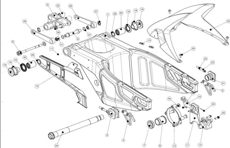
Swingarm
